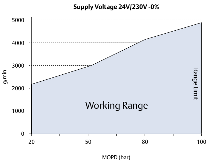
Fig. 1: Performance related to supply voltage: Flow Rate and Differential Pressure between inlet and outlet (Oil type Renisco C85E, oil temperature 54°C)
