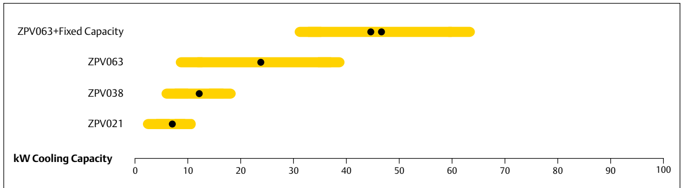
Copeland Scroll™ ZPV063 Variable Speed compressor and drive
